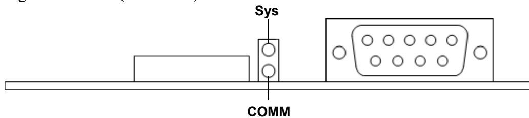
Figure 3: LEDs (Side View)
