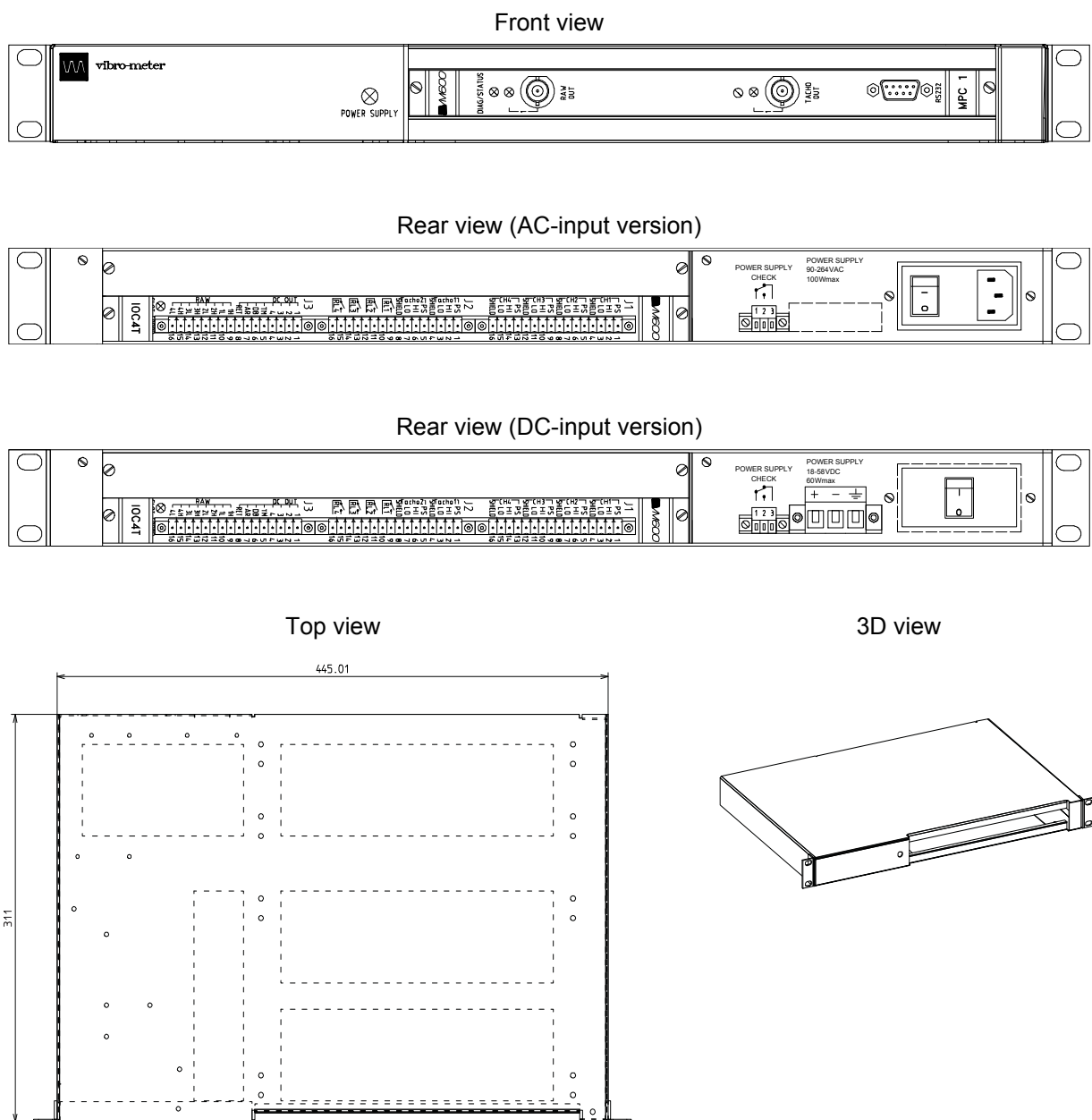
Figure 2-4: Views of a typical ABE056 rack
