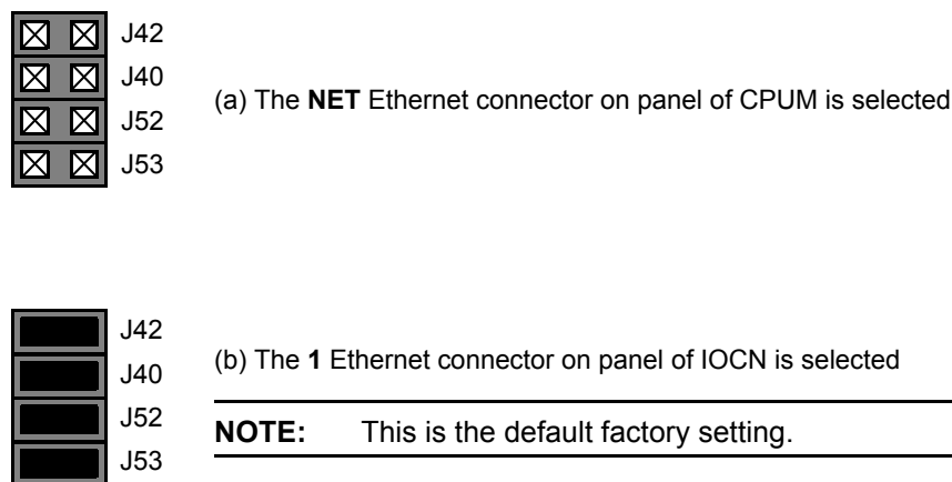
Figure 13-1: CPUM card jumper settings to select the Ethernet connector
