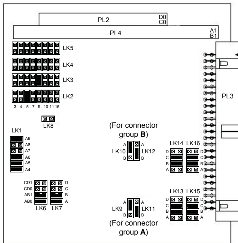
Figure 13-8: Serial communications module jumper settings to select full-duplex RS-485 communications for earlier versions of the CPUM card (MSM586EN or equivalent)
