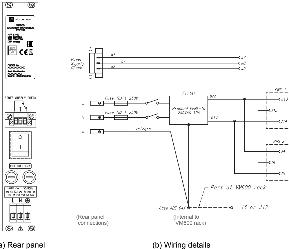
Figure 2-21: AC-input (120/230 V AC ) panel with a common input (screw-terminal connector and on/off switch)
