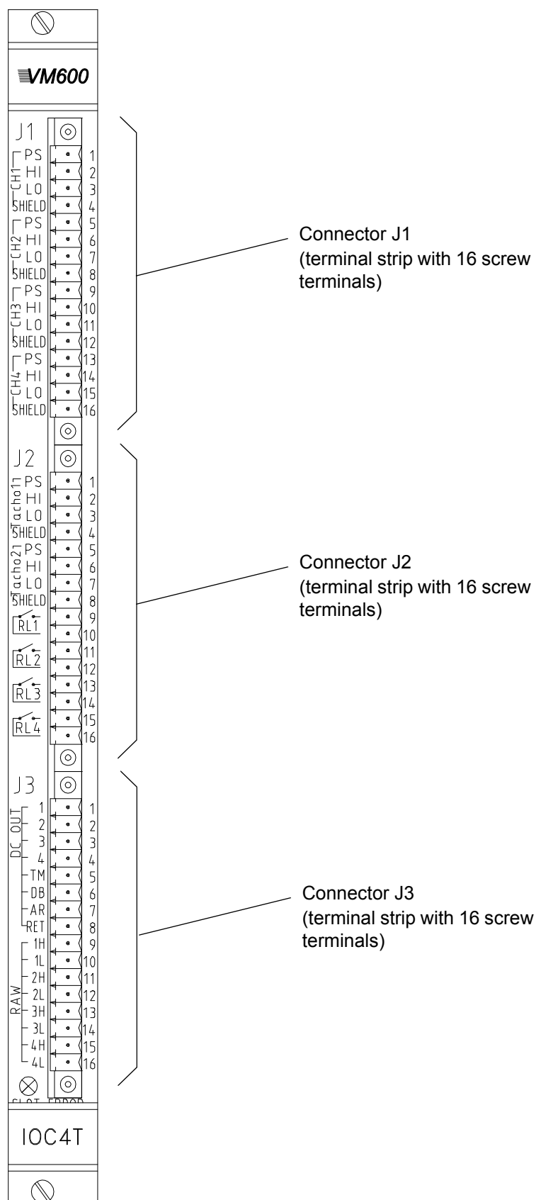
Figure 9-1: View of IOC4T card showing definition of terminals
