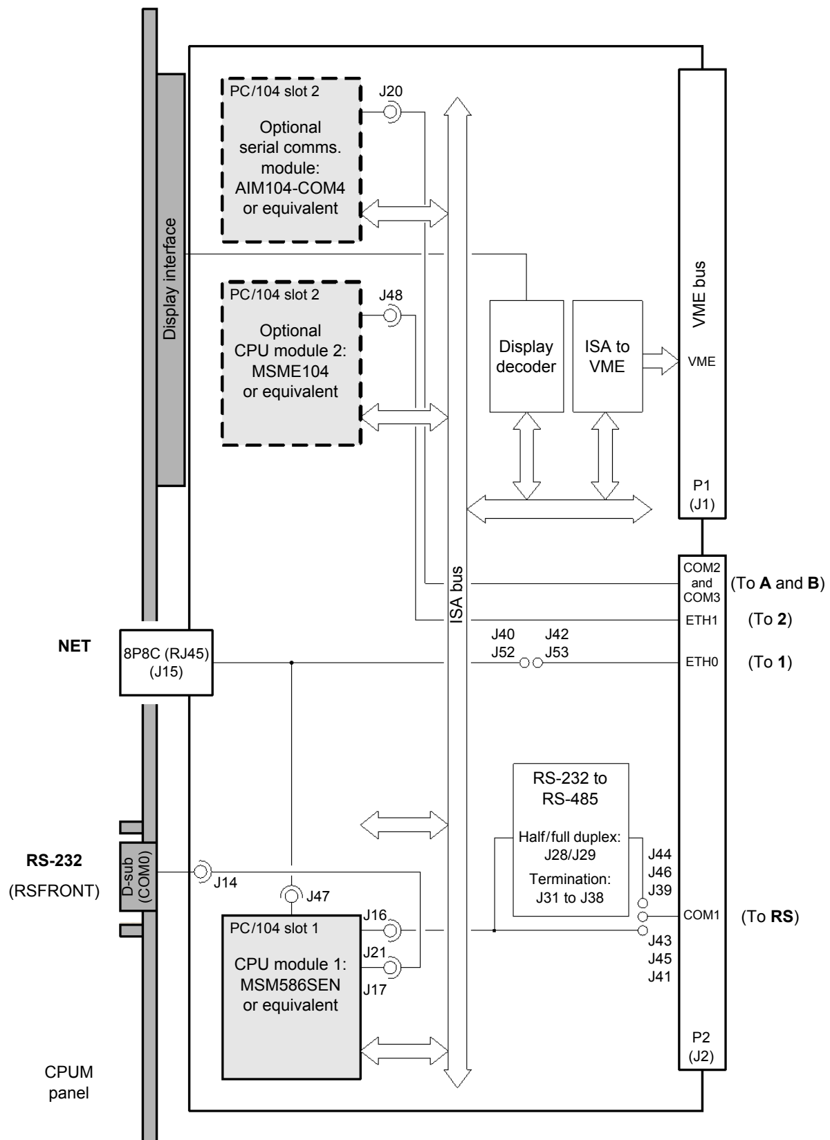
Figure 6-2: Block diagram of CPUM card fitted with the MSM586SEN or equivalent CPU module (PNR 200-595-075-HHh or earlier)
