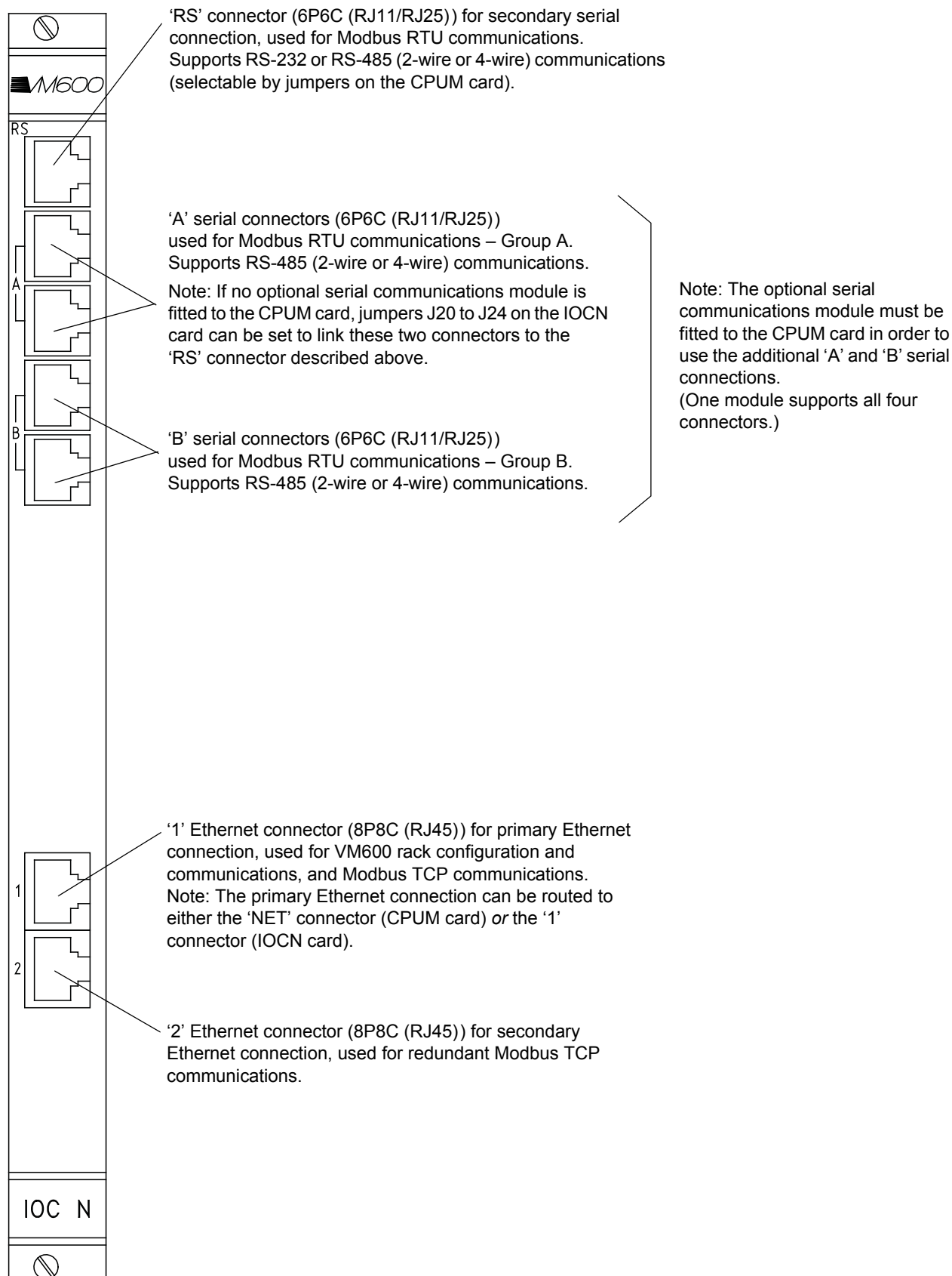
Figure 2-12: Elements on the IOCN
