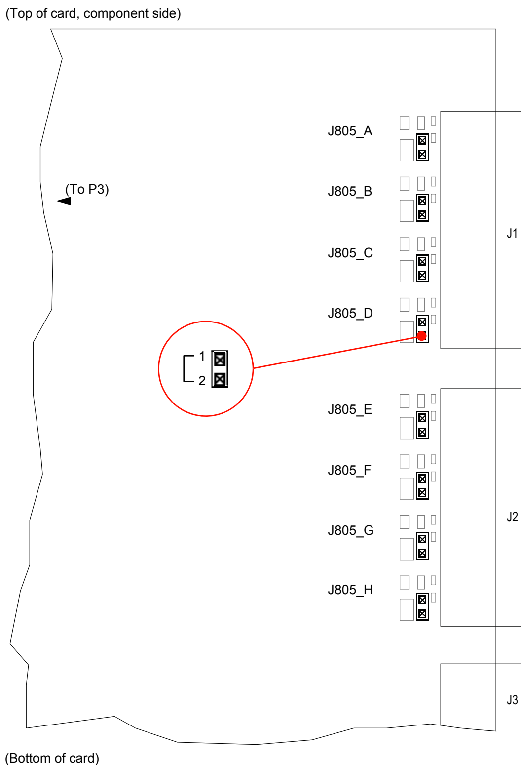
Figure 10-3: Position of jumpers J805_x on IOC8T card
