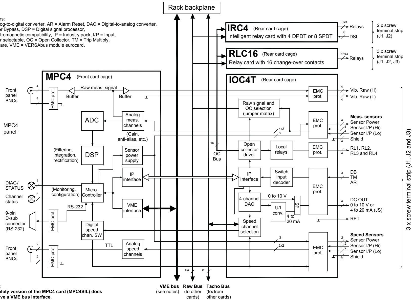
Figure 4-2: Block diagram of MPC4, IOC4T, RLC16 and IRC4 cards
