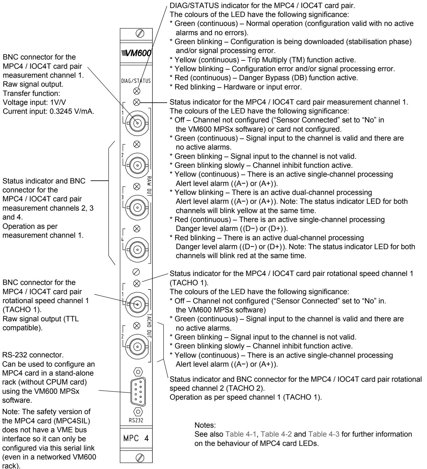
Figure 2-7: Elements on the MPC4
