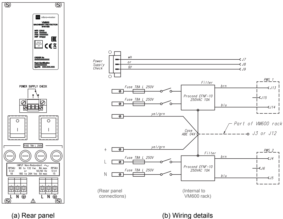
Figure 2-24: AC-input (120/230 V AC ) panel with individual inputs (screw-terminal connectors and on/off switches)
