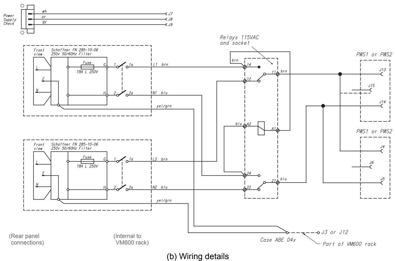
Figure 2-26: AC-input (120 V AC only) panel with individual inputs supporting external mains power supply redundancy
