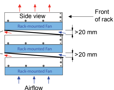
Figure 8-2: Minimum required spacing above, below and between ABE056 racks in an enclosure using natural or forced ventilation
