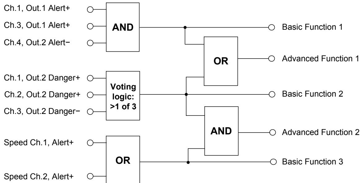
Figure 4-7: Example showing basic and advanced logic functions
