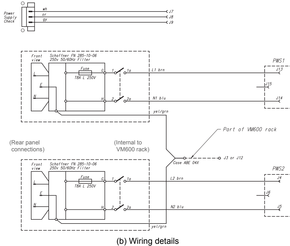
Figure 2-23: AC-input (120/230 V AC ) panel with individual inputs (mains sockets and on/off switches)
