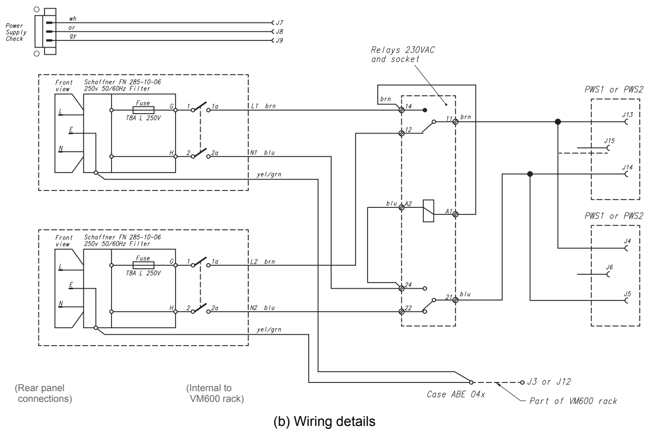
Figure 2-27: AC-input (230 V AC only) panel with individual inputs supporting external mains power supply redundancy
