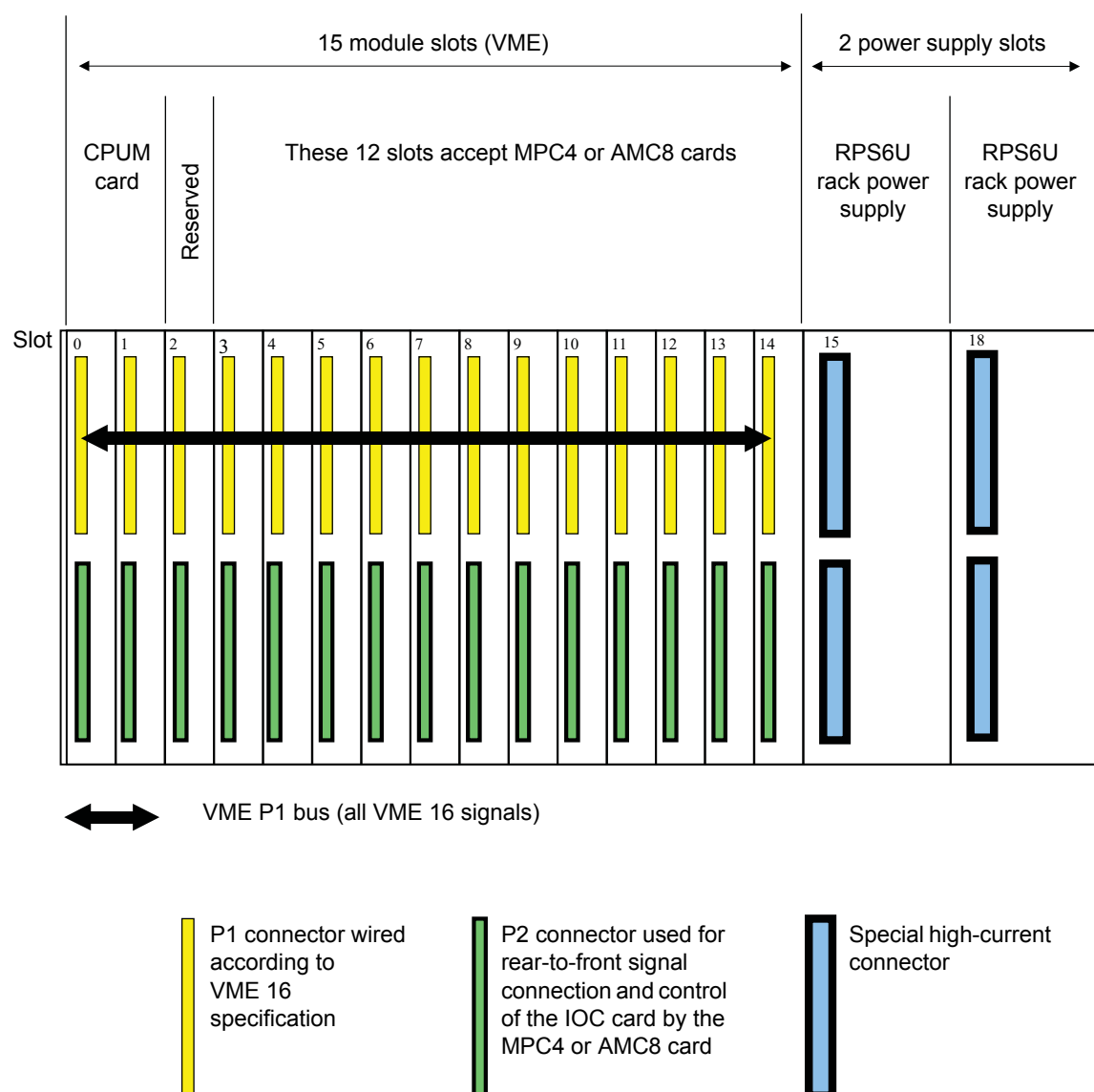
Figure 3-4: Diagram of VM600 rack (ABE04x) backplane showing the arrangement of the connectors
