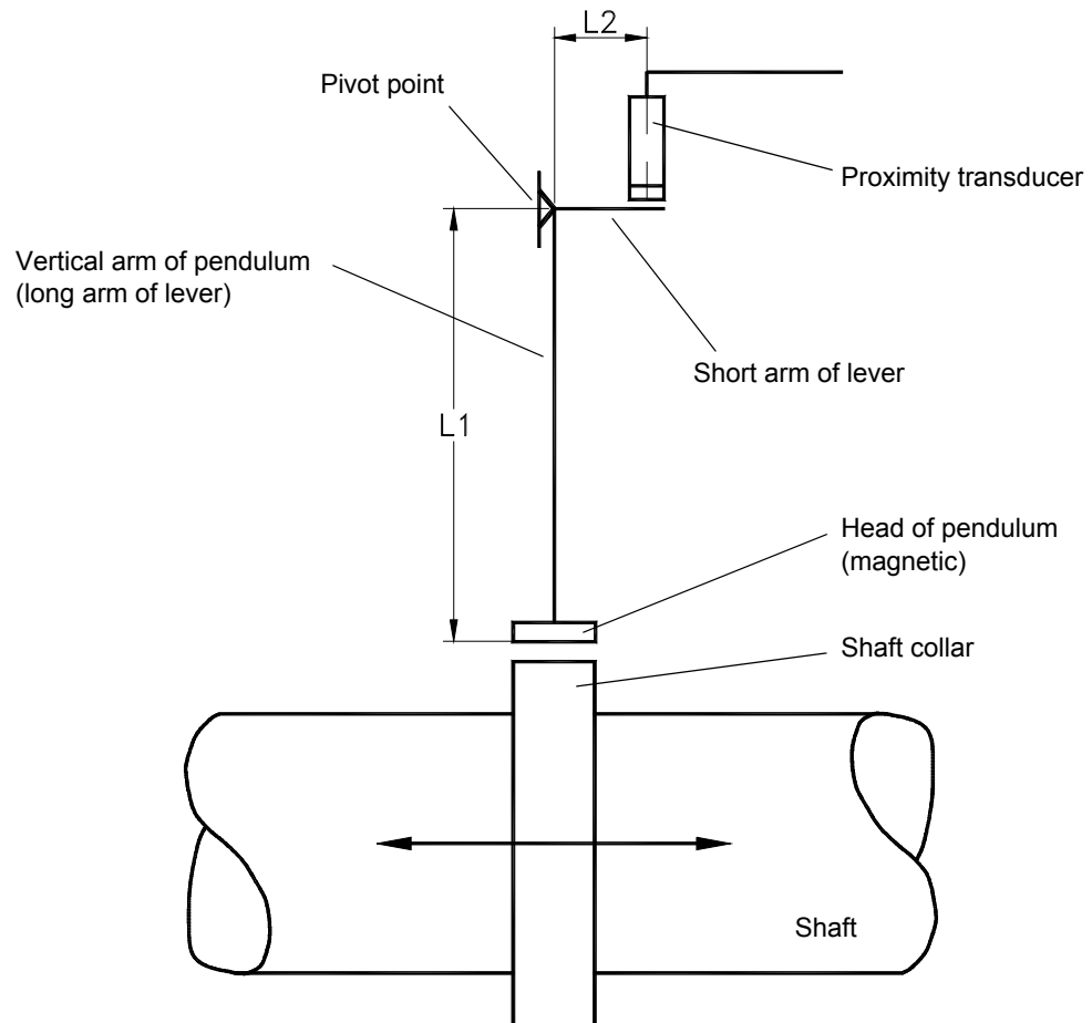
Figure 7-17: A measuring system using a pendulum with magnetic head installed near a shaft collar
