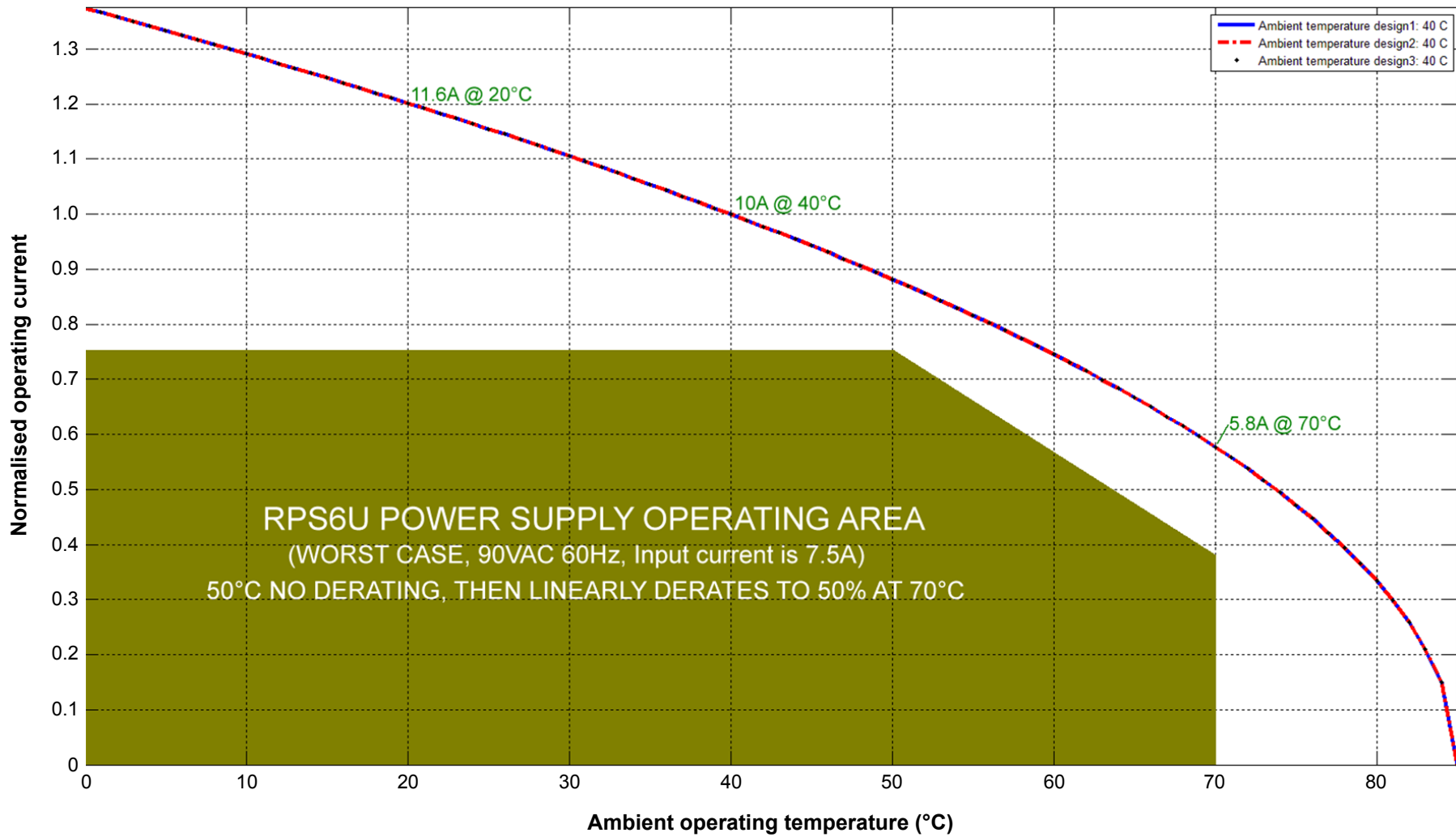
Figure A-1: Temperature derating for the power entry module (AC input) of a VM600 rack
