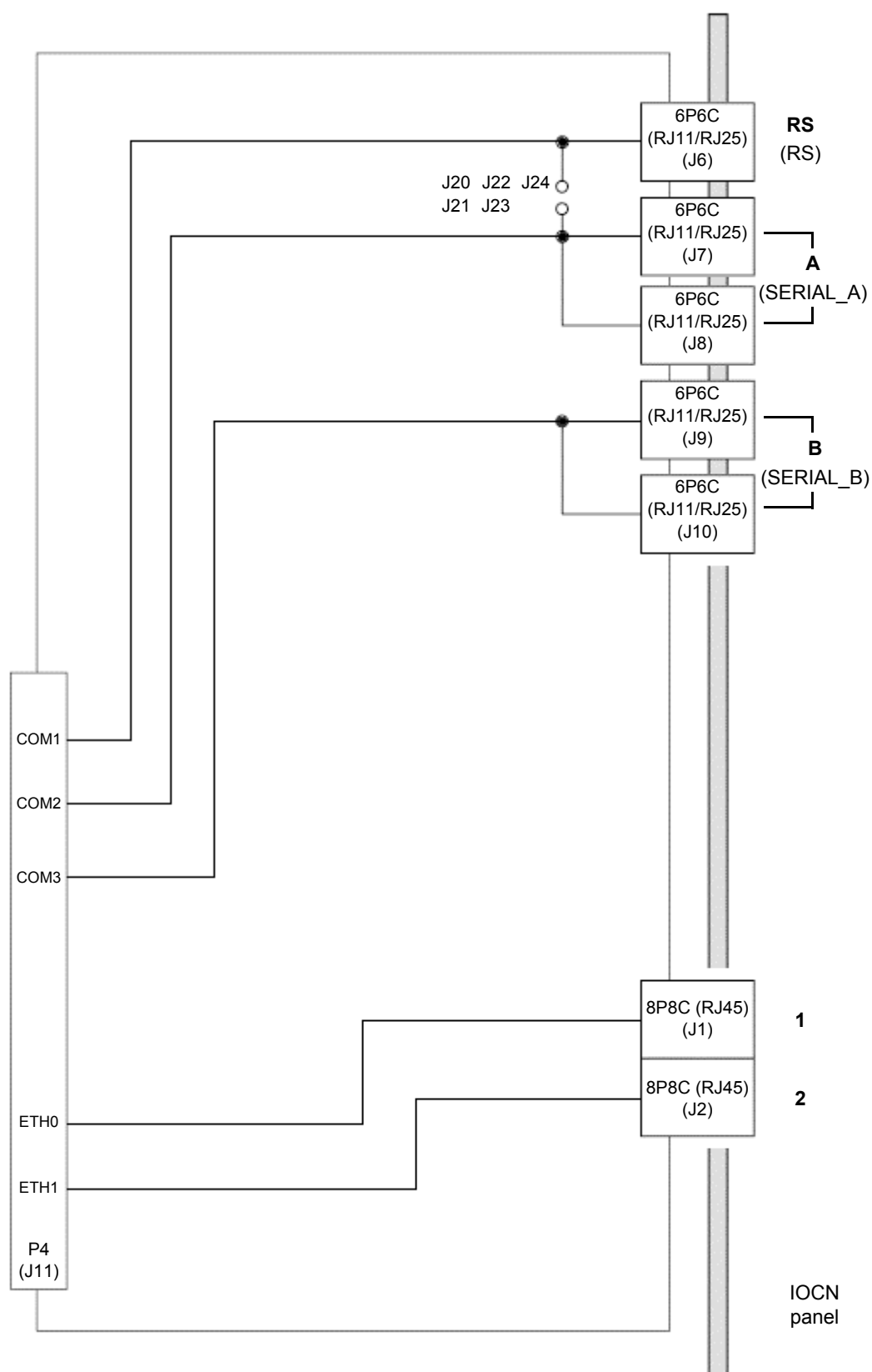
Figure 6-3: Block diagram of IOCN card
