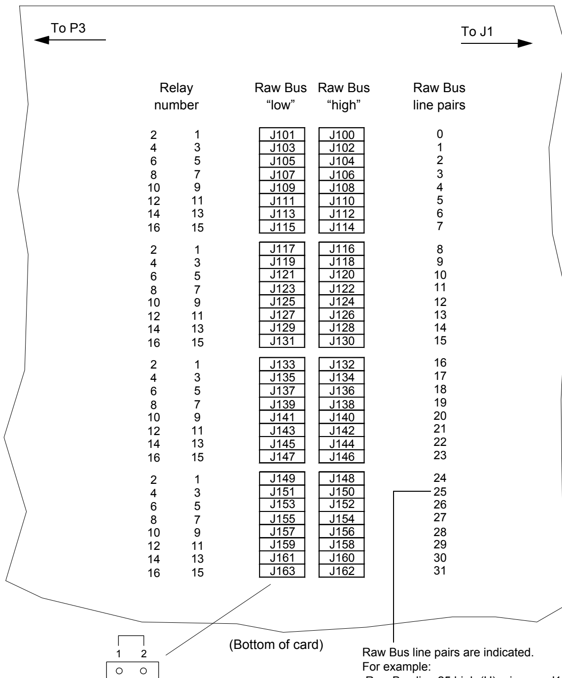
Figure 10-18: Position of jumpers on the IOC8T card related to the Raw Bus lines
