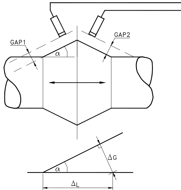
Figure 7-13: Two proximity probes mounted near a shaft fitted with a double taper
