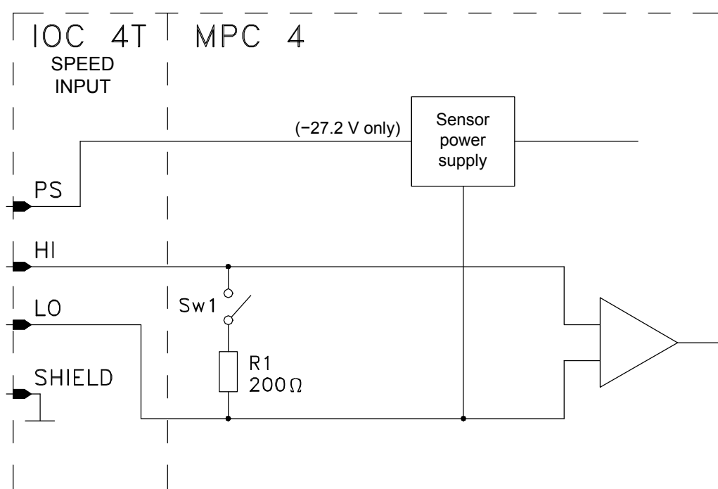
Figure 9-15: Circuitry associated with speed channel inputs
