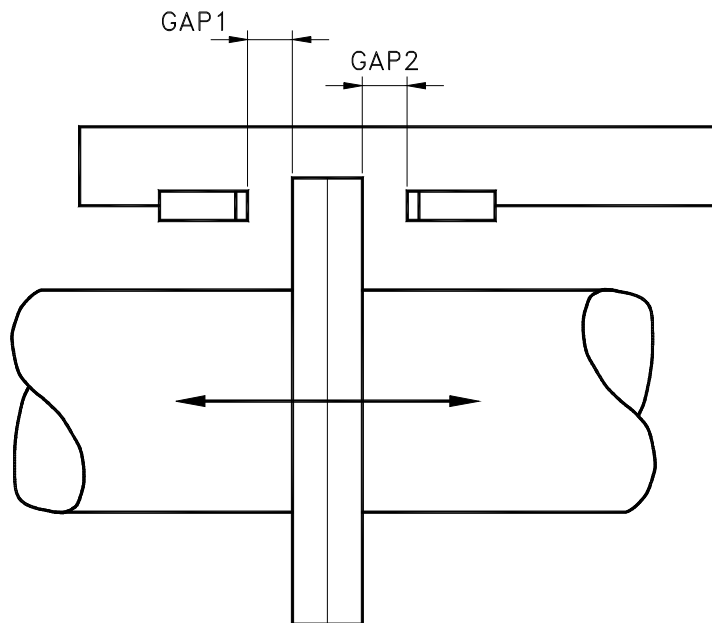
Figure 7-11: Two proximity probes mounted near a shaft fitted with a collar
