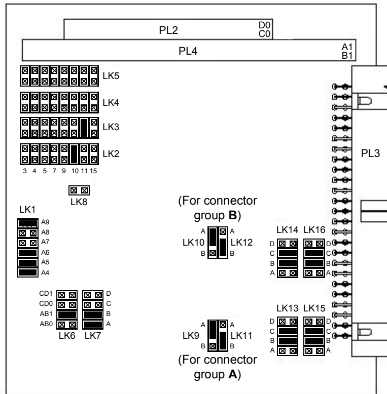
Figure 13-7: Serial communications module jumper settings to select full-duplex RS-485 communications for later versions of the CPUM card (PFM-5411 or equivalent)
