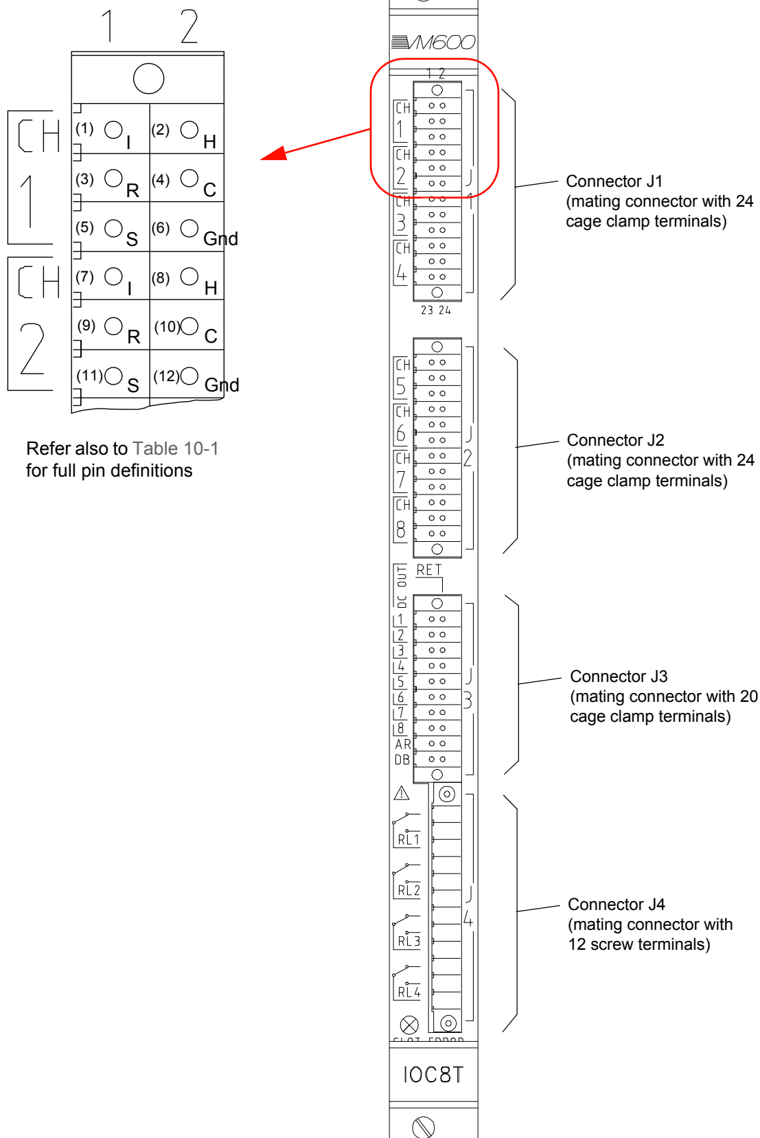
Figure 10-1: View of IOC8T card showing definition of terminals (without mating connectors)
