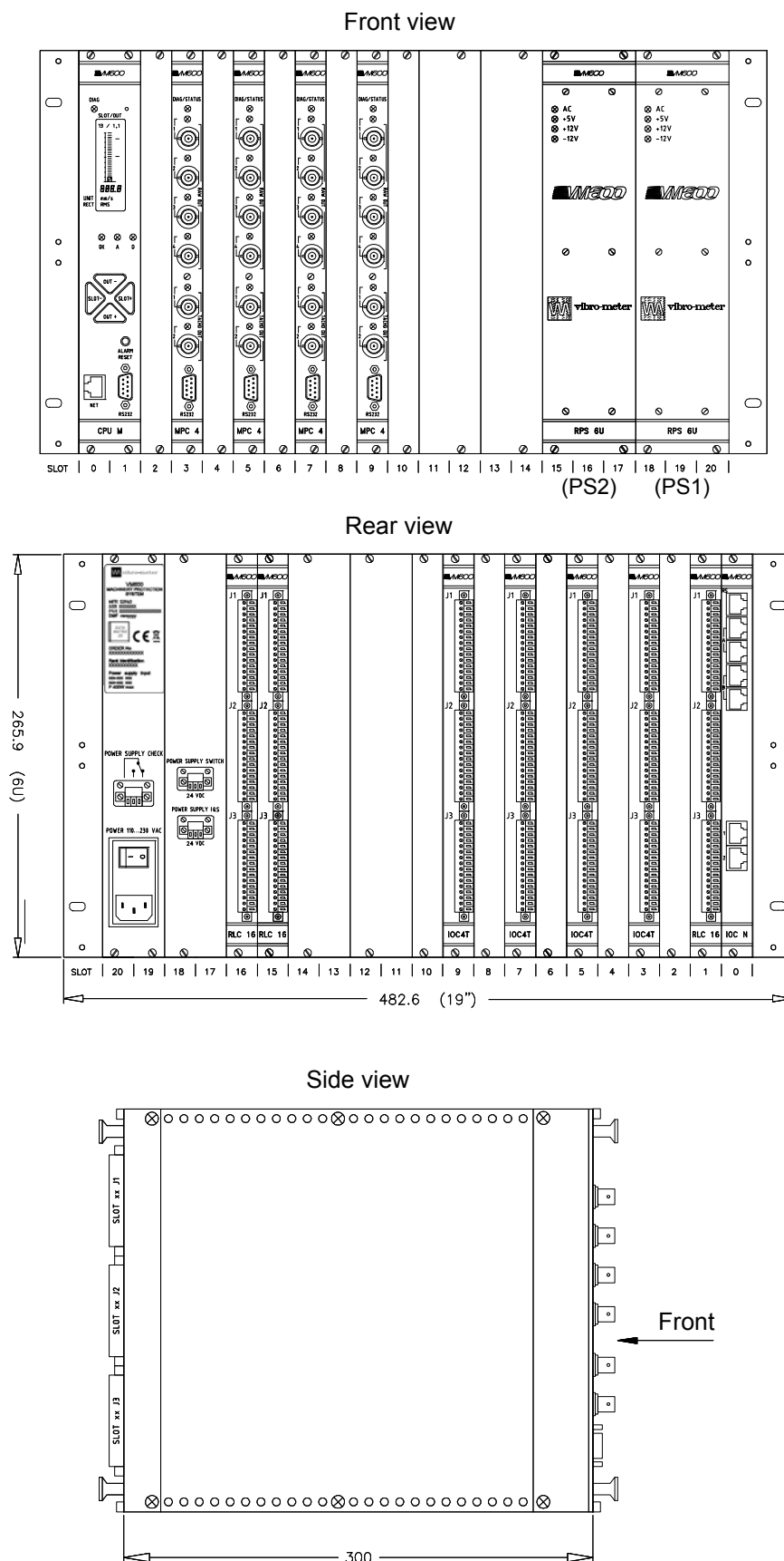
Figure 2-1: Views of a typical ABE040 rack with several cards installed (machinery protection cards only)
