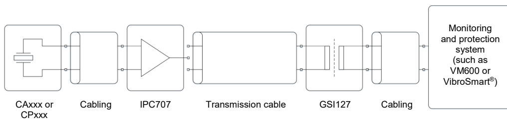
IPC707 output signal
