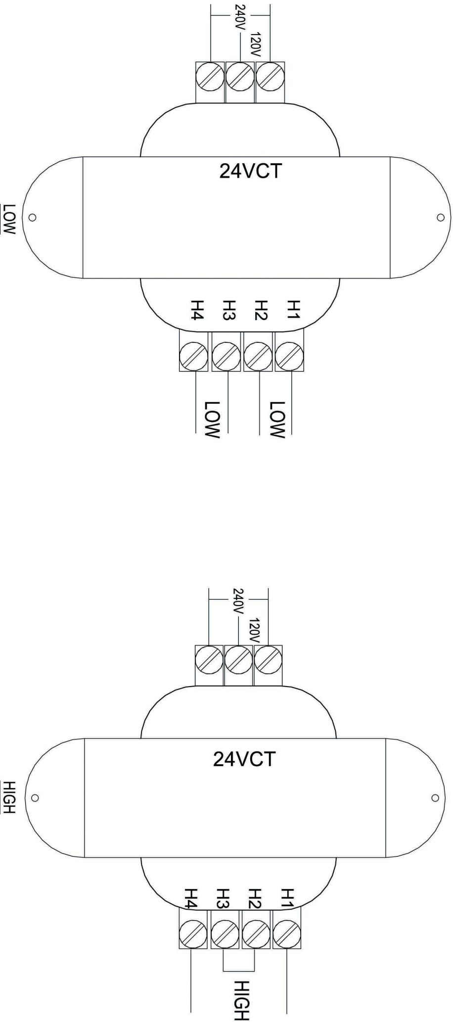
TRANSFORMER 120V/240 to 24VCT 20VA OPEN TYPE
