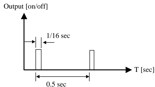
Figure 1: AB1A output in Step mode
