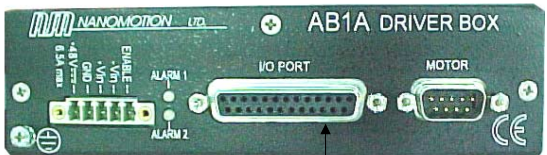
Figure 4: AB1A Box Front Panel
