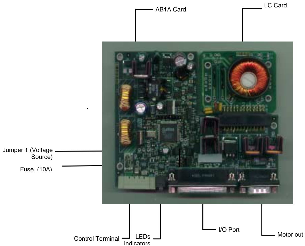
Figure 7: AB1A Card
