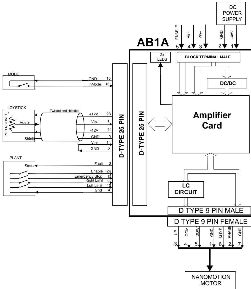
Figure 12: Joystick Interface
