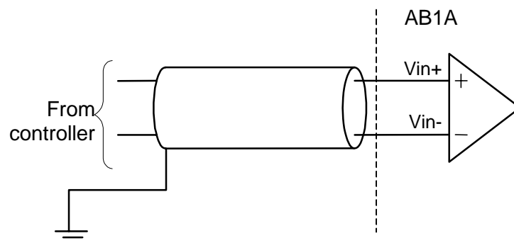
Figure 5: Differential Analog Input Connection
