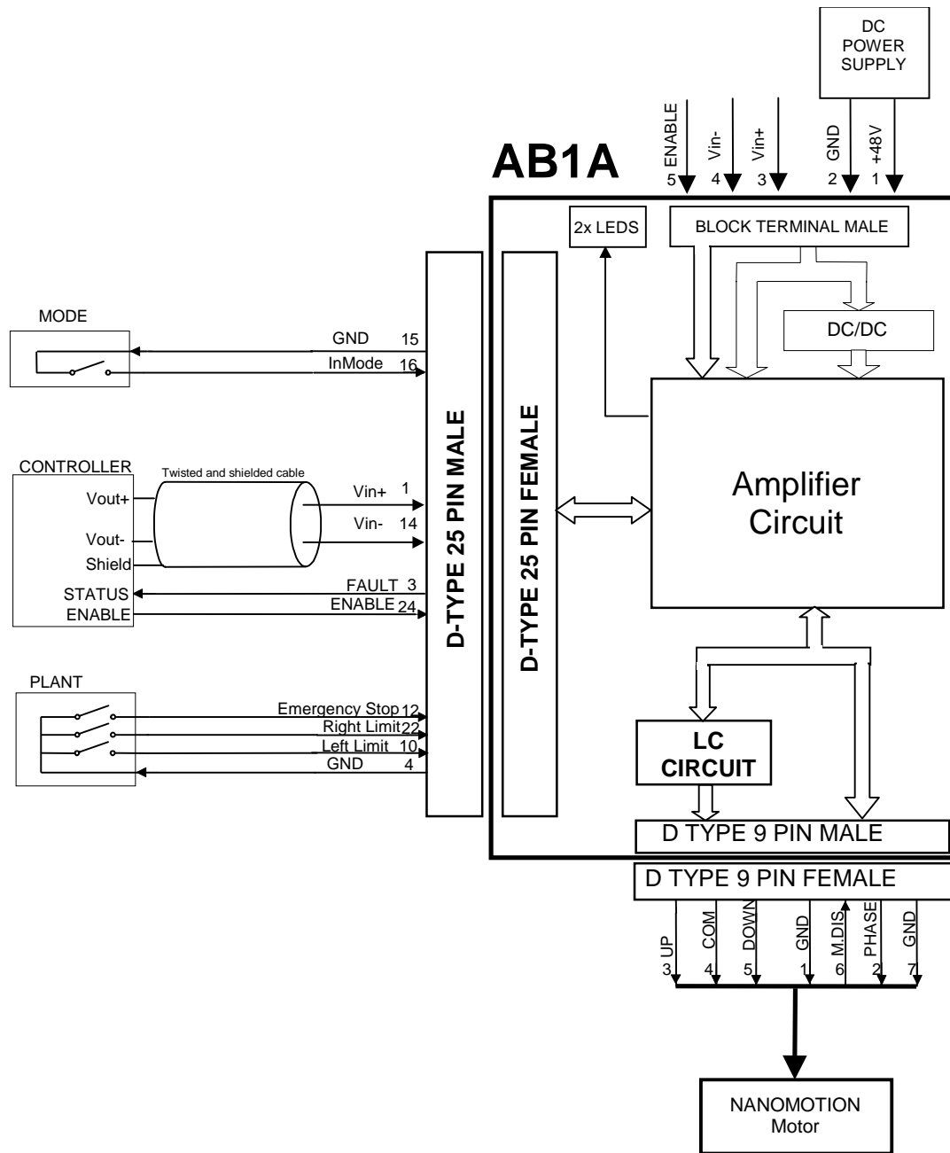
Figure 11: Differential Interface
