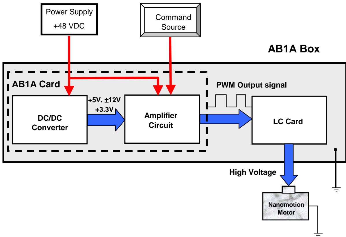
Figure 2: AB1A Block Diagram
