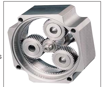
Figure 2 - Ring gear is cut directly into the main housing of a Stealth Planetary gearhead.
